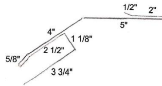
S.S Upper Gambrel
