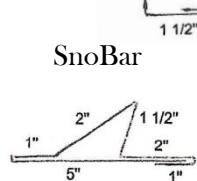
SnoBar
