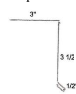
3.5 Gutter Apron
