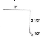
2.5 Gutter Apron
